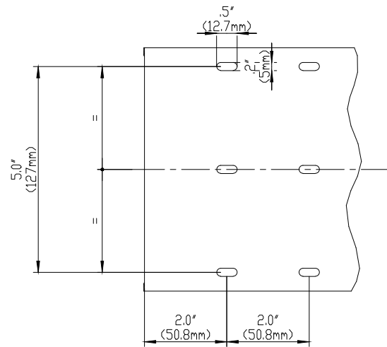
BASE PERFORATION
