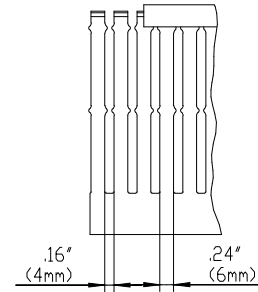
SIDE SECTION
