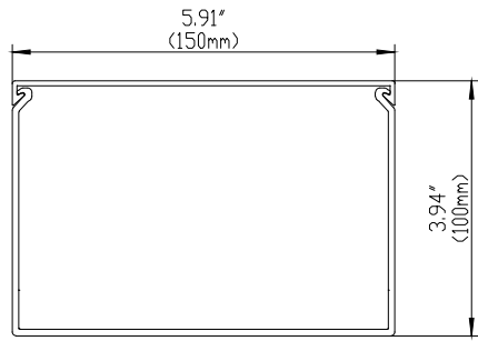
FRONT SECTION
