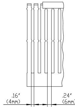
SIDE SECTION
