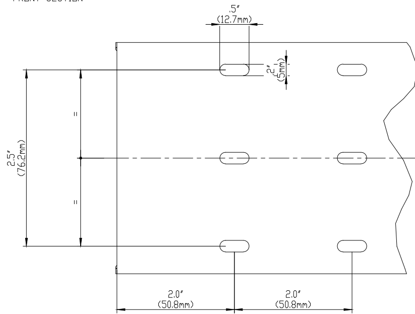
BASE PERFORATION
