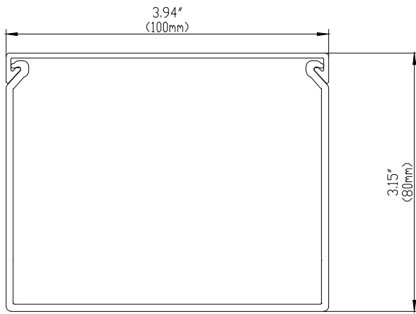
FRONT SECTION
