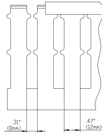
SIDE SECTION
