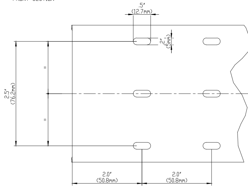
BASE PERFORATION
