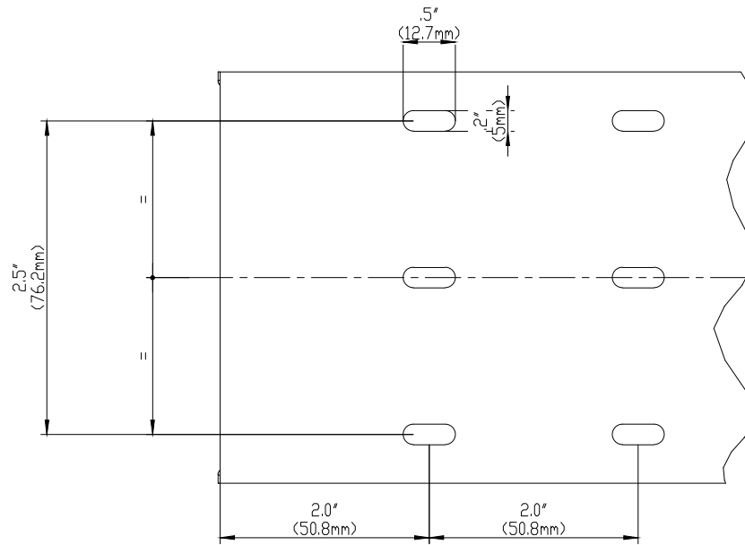
FRONT SECTION
