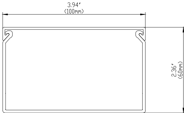
FRONT SECTION
