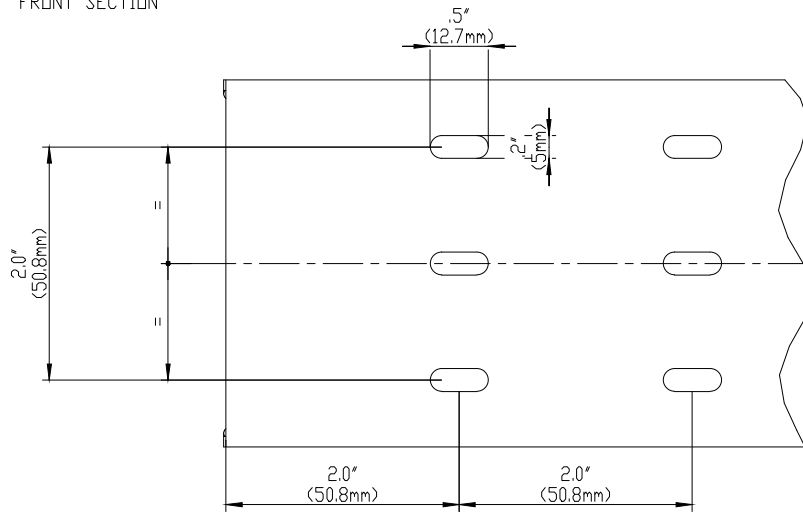
BASE PERFORATION
