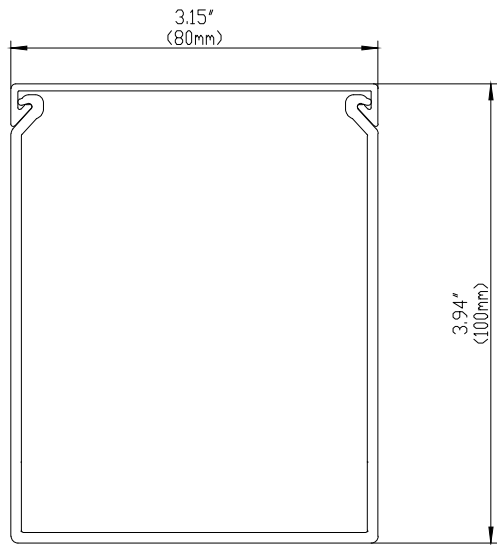
FRONT SECTION
