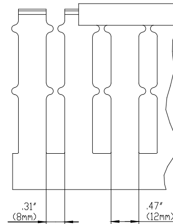
SIDE SECTION
