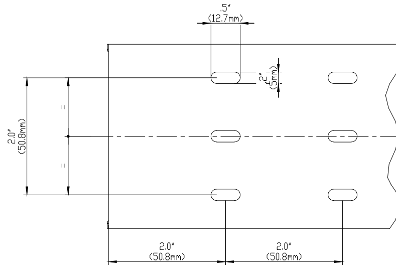
BASE PERFORATION
