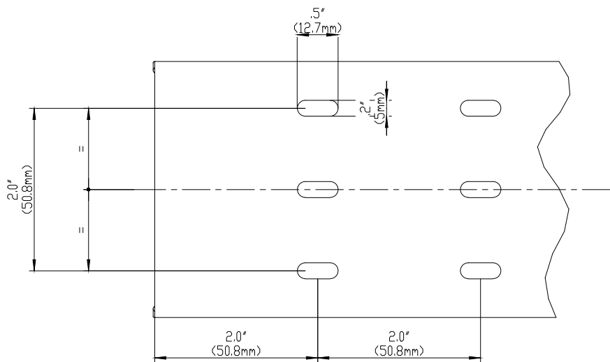
BASE PERFORATION
