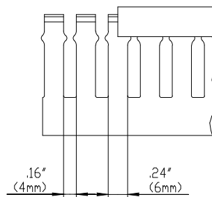
SIDE SECTION
