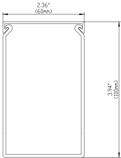
FRONT SECTION
