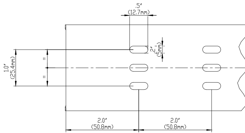
BASE PERFORATION
