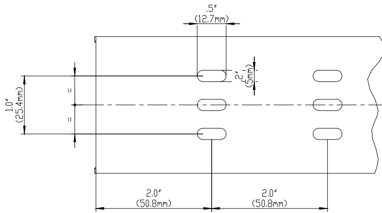
BASE PERFORATION
