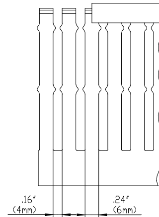
SIDE SECTION
