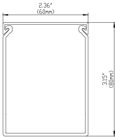
FRONT SECTION
