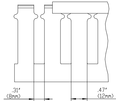
SIDE SECTION
