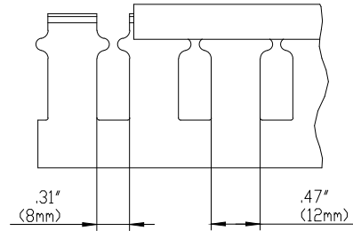
SIDE SECTION
