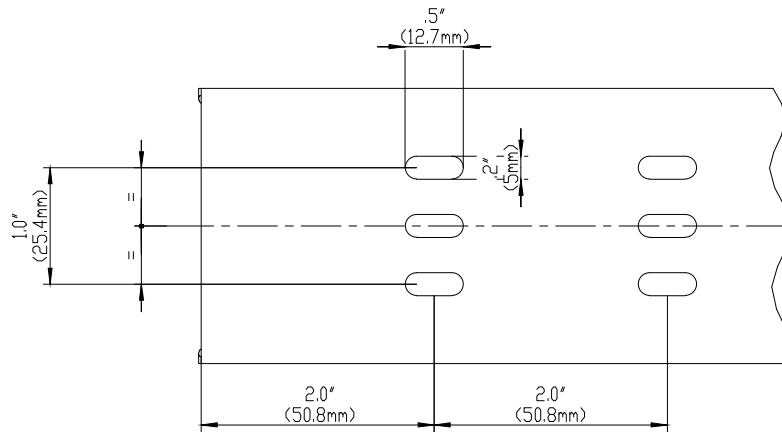
BASE PERFORATION
