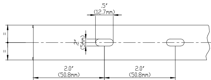
BASE PERFORATION
