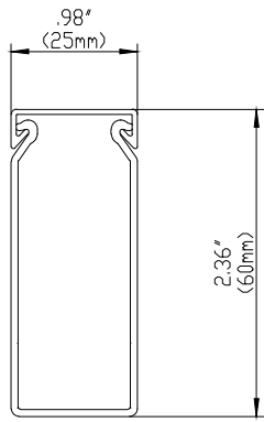
FRONT SECTION
