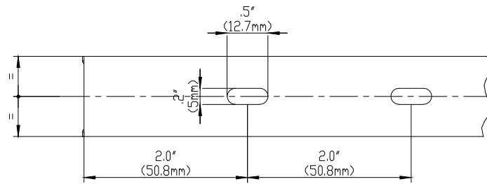
BASE PERFORATION
