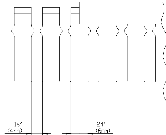
SIDE SECTION
