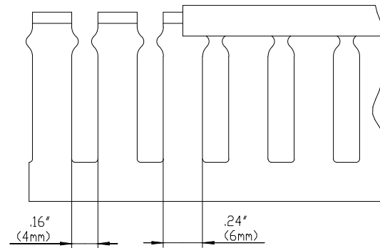
SIDE SECTION
