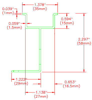
FRONT SECTION
