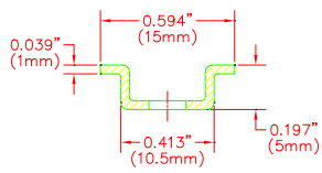
FRONT SECTION
