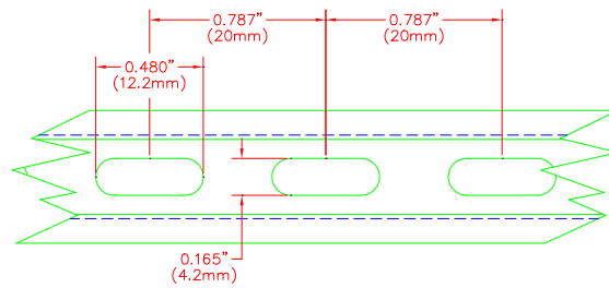
BASE PERFORATION
